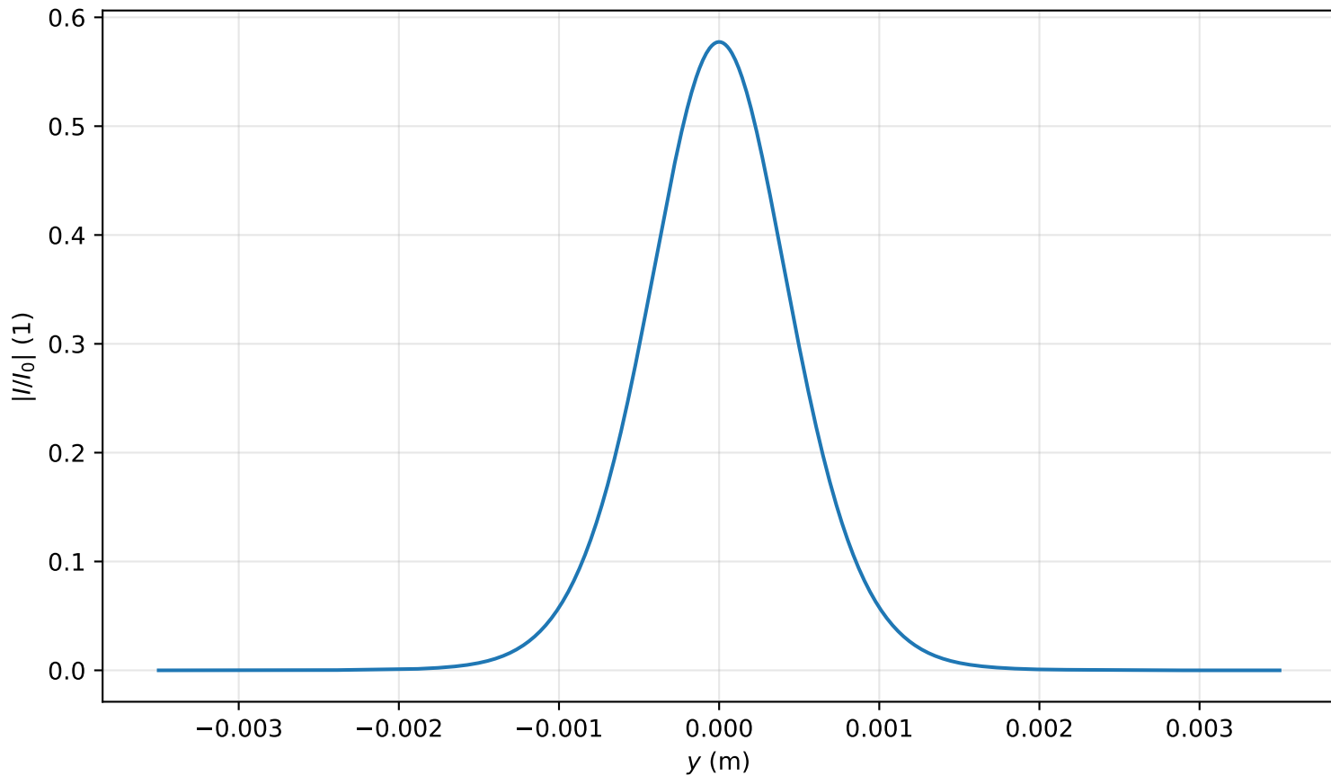
Intensity profile I(x=0, y, z=2.946)/I_0 , \text{Pin}=0.5\text{Pcr} , artificial time
